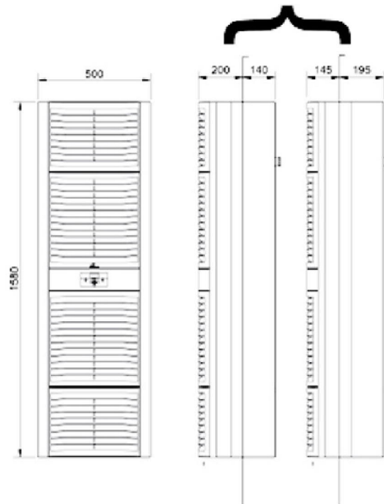
door mounting
